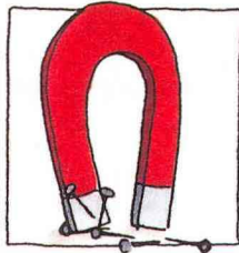
magnet
