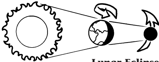
Lunar Eclipse
